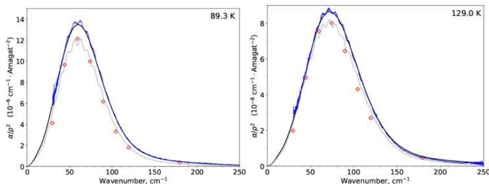
Fig. 35. \text{N}_2\text{-N}_2 collision-induced absorption spectra at two temperatures. The black curves indicate results from the trajectory-based calculation [789], the blue curves denote the experimental measurements [792], the red diamonds denote the results from the quantum-mechanical calculation [806], and the grey curves denote Borysow model spectra [810]. (For interpretation of the references to color in this figure legend, the reader is referred to the web version of this article.)
