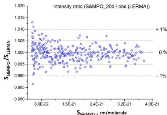
Fig. 12. Ratio of intensities S(\text{S\&MPO}_{20\text{d}}) / S(\text{LERMA}_{\text{obs}}) for the strongest lines in the 5- \mu\text{m} range. Note that the S&MPO data are used in HITRAN2020 in this spectral region.
