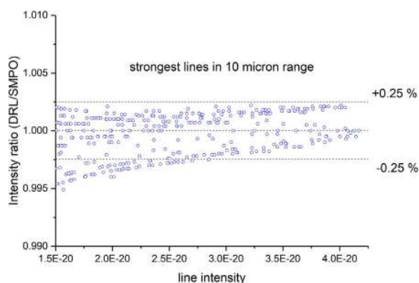
Fig. 11. Ratio of intensities S(\text{DLR})/S(\text{S\&MPO}_{20\text{d}}) for the strongest lines in the 10- \mu\text{m} range. Note that the DLR data are used in HITRAN2020 in this spectral region.
